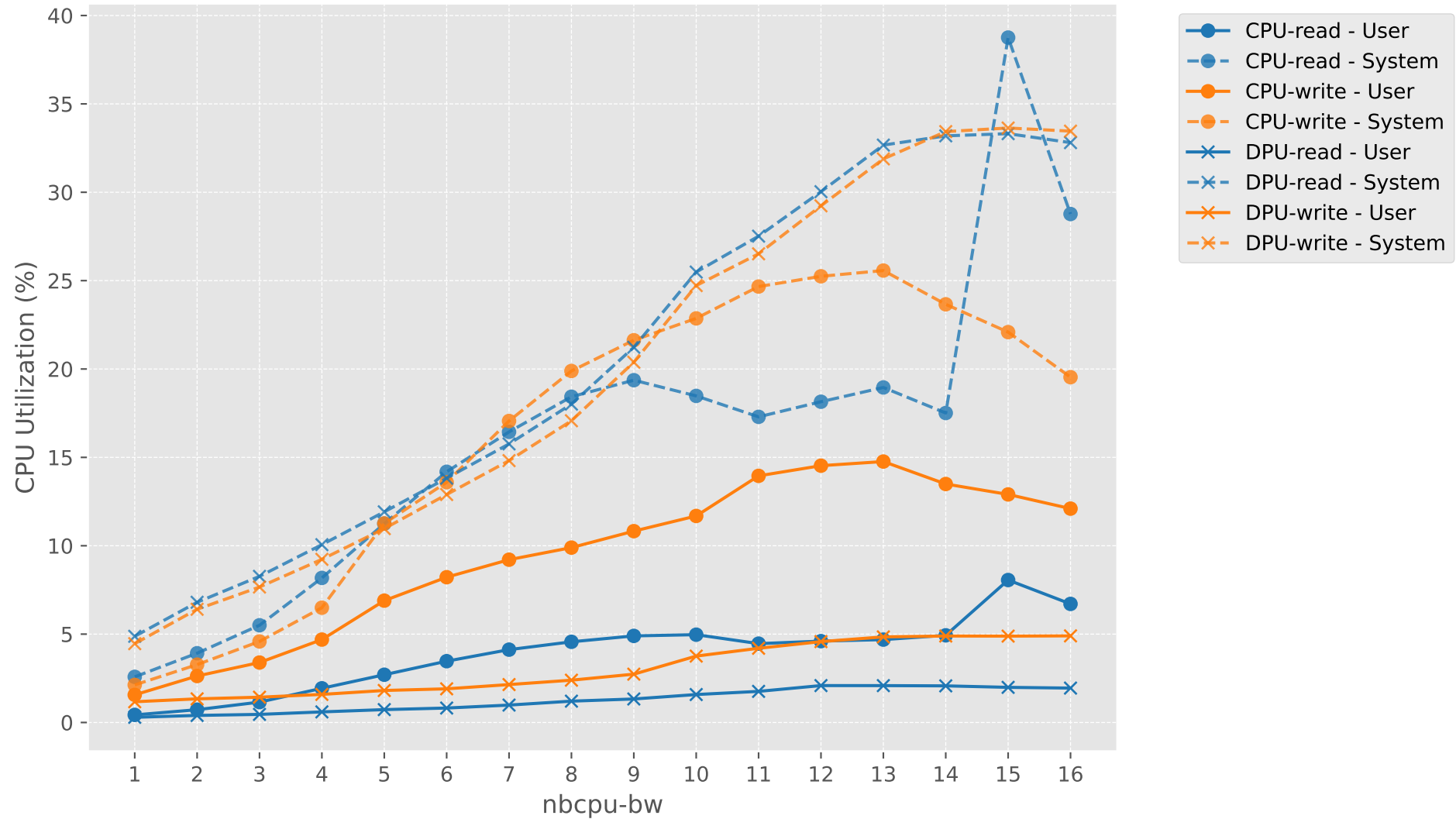
CPU Utilization vs nbcpu-bw
